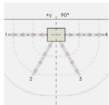
Top view (from EXPERT software)
