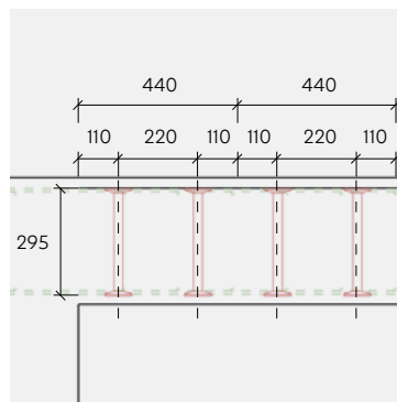
Cross section (from EXPERT software)
