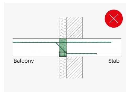
ISOPRO®IP - Incorrect installation, shear bar must be at the bottom on the balcony side
