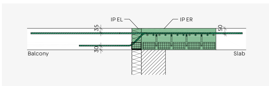
ISOPRO® IP Corner – Cross-section of corner situation
