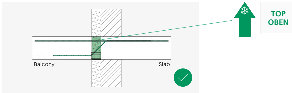
ISOPRO® IP – Correct installation
