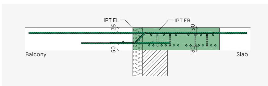
ISOPRO® IPT Corner – Cross-section of corner situation
