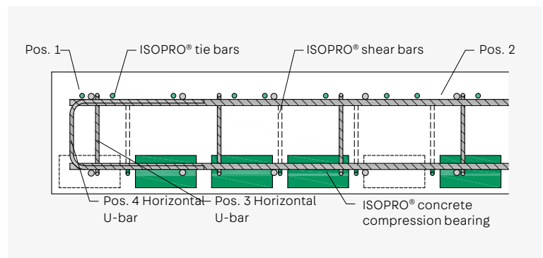
ISOPRO® IP - Cross section A-A
