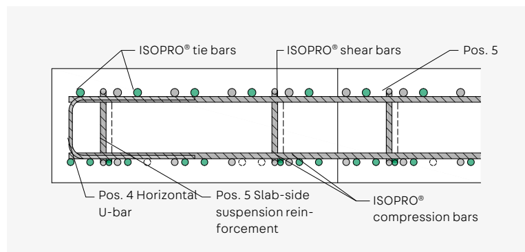
ISOPRO® IPT – Cross section A-A
