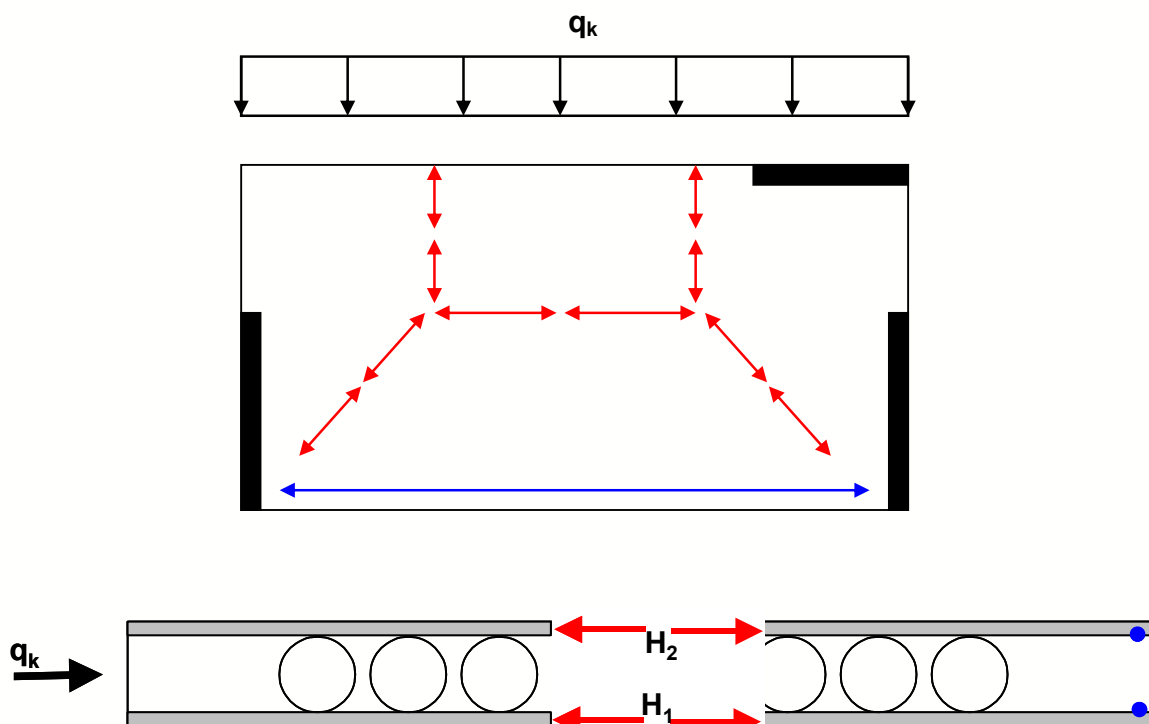
Figure 12 – Comportement Diaphragme de la Dalle Cobiax
