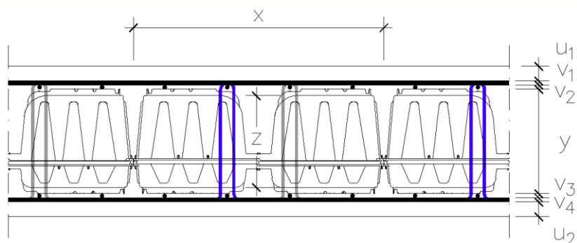
Figure 6 – Section type d'une dalle COBIAX CLS.
