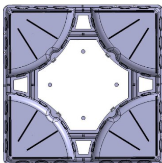
Figure 1 – Module COBIAX CLS
