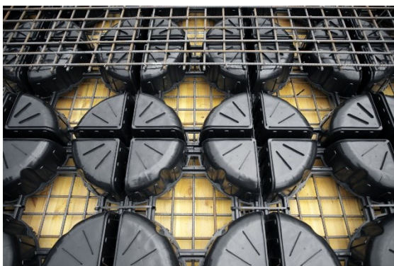
Figure 2 – Dalle COBIAX CLS
