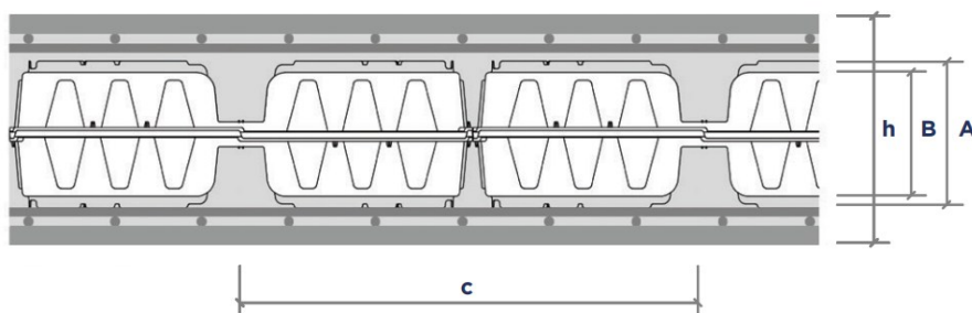
Figure 5 – Section type d'une dalle COBIAX CLS.
