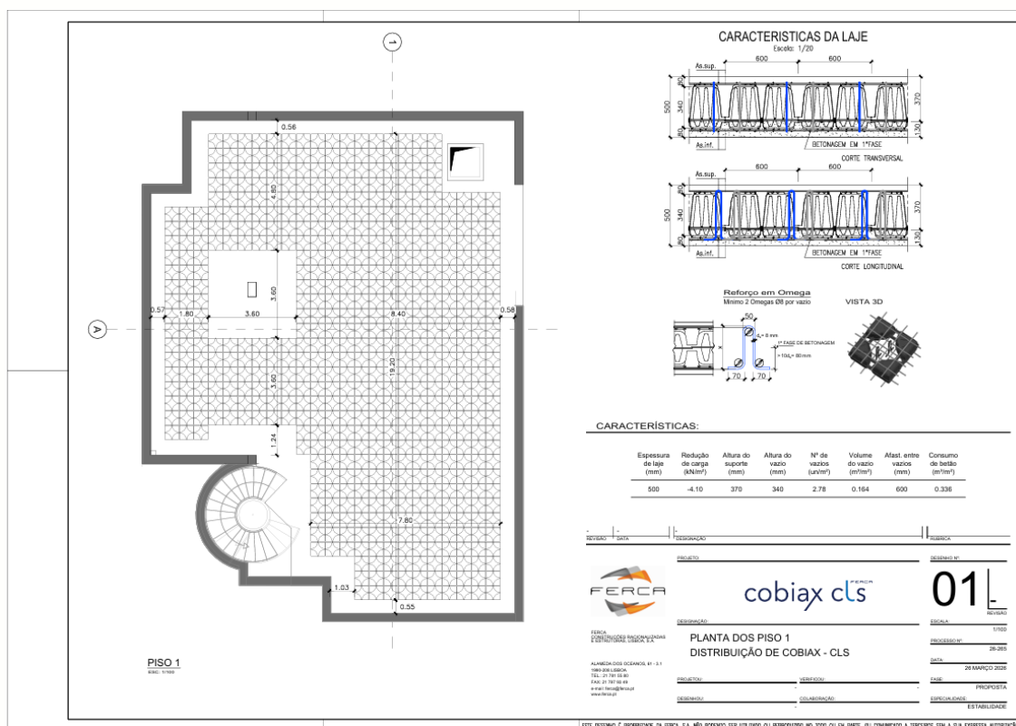
Figura 15 – COBIAX CLS layout drawing
