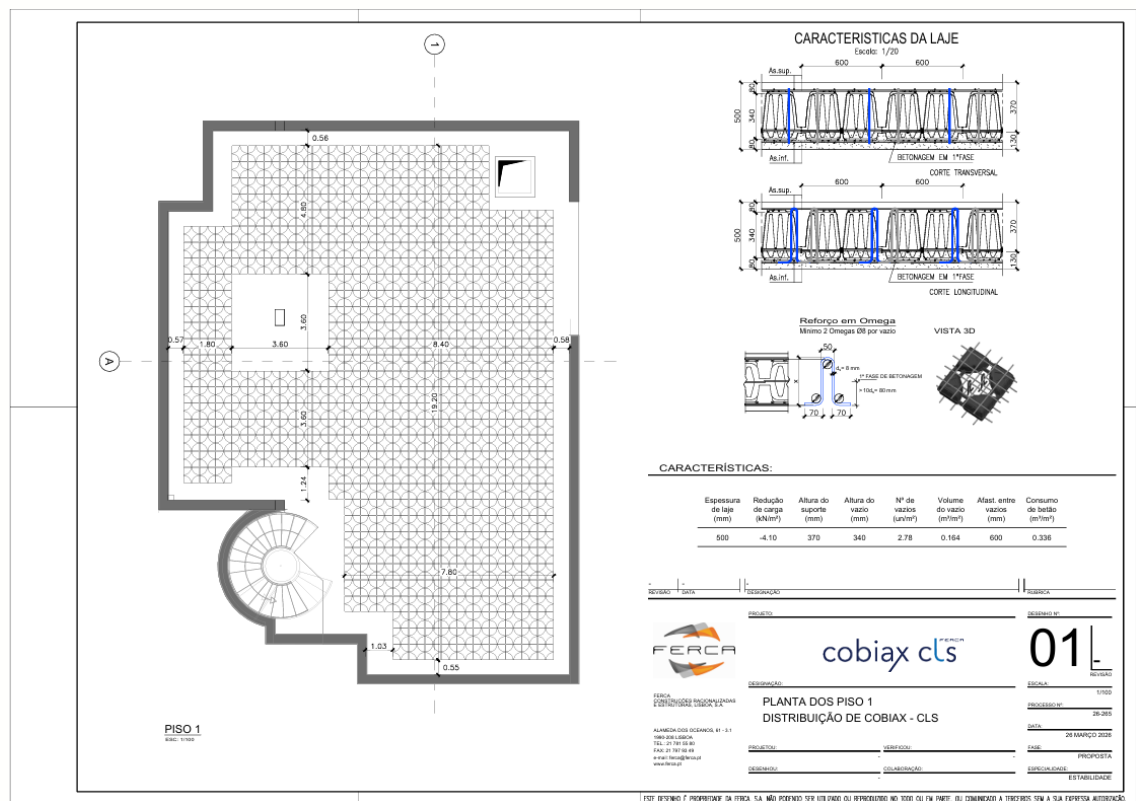
Figure 15 – COBIAx CLS layout drawing
