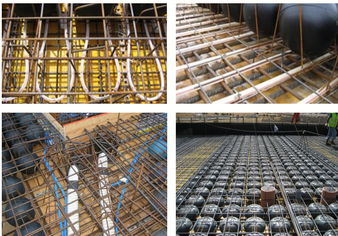
Figure 16 -Examples of various services and post-tensioning systems in a COBIAX CLS slab
