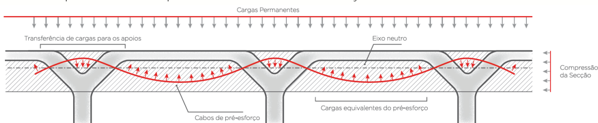
Figure 14 – Equivalent prestress loads on the COBIAX CLS slab
