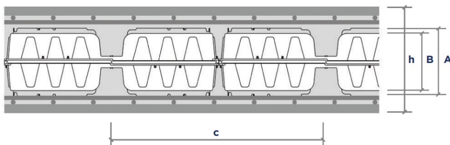
Figure 5 – Typical section of a COBIAX CLS slab.
