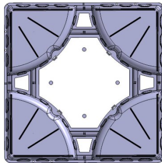
Figure 1 – COBIAX CLS module
