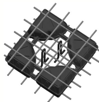
Figure 9 – Position of the omegas within zone X
