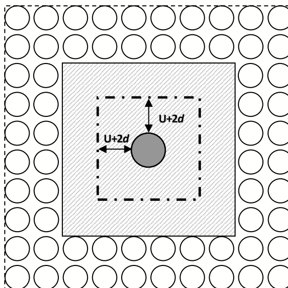
Figure 10 – Solid zone due to punching shear
