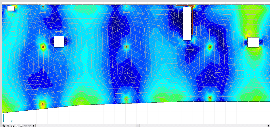
Distribution of forces at ultimate limit states
