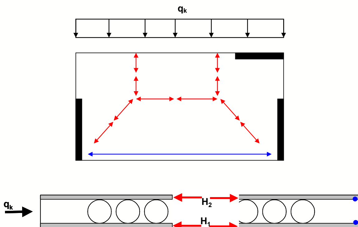
Figure 12 – Diaphragm behaviour of the COBIAX slab
