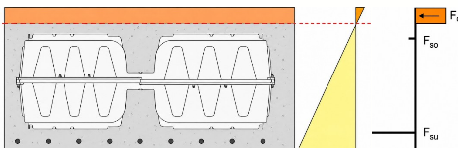
Figure 7 – Position of the neutral axis above the void within the compression layer.
