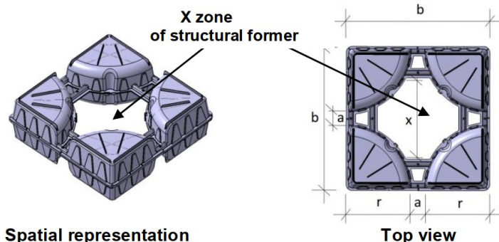
Figure 8 – Definition of zone X
