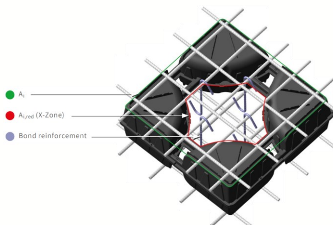
Figure 11 – Example of reinforcement in zone X of a COBIAx CLS slab
