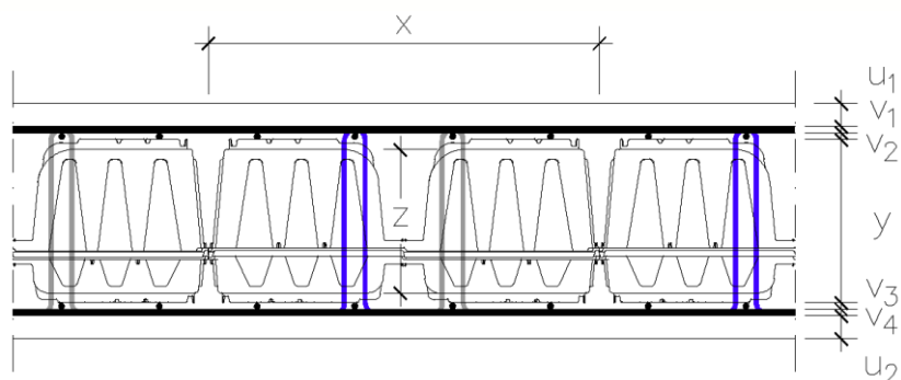
Figure 6 – Typical section of a COBIAX CLS slab.
