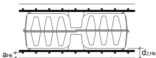
Figure 13 – Relevant distances for fire resistance
